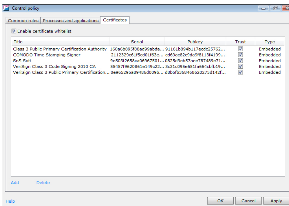
Figure 56. The white list of certificates
