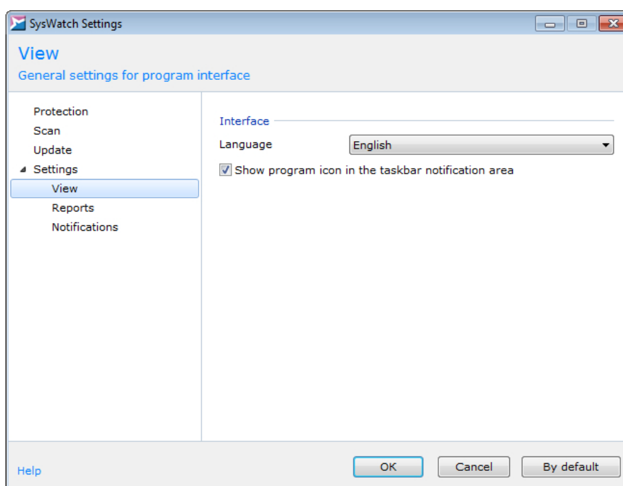
Figure 33. Interface settings
