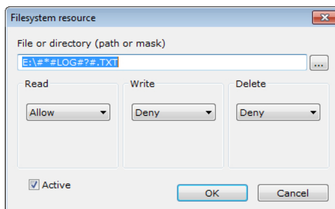
Figure 59. Creating a rule for the file system object
