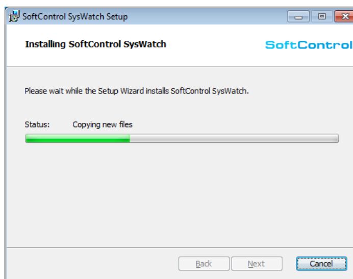
Figure 6. Installation progress
