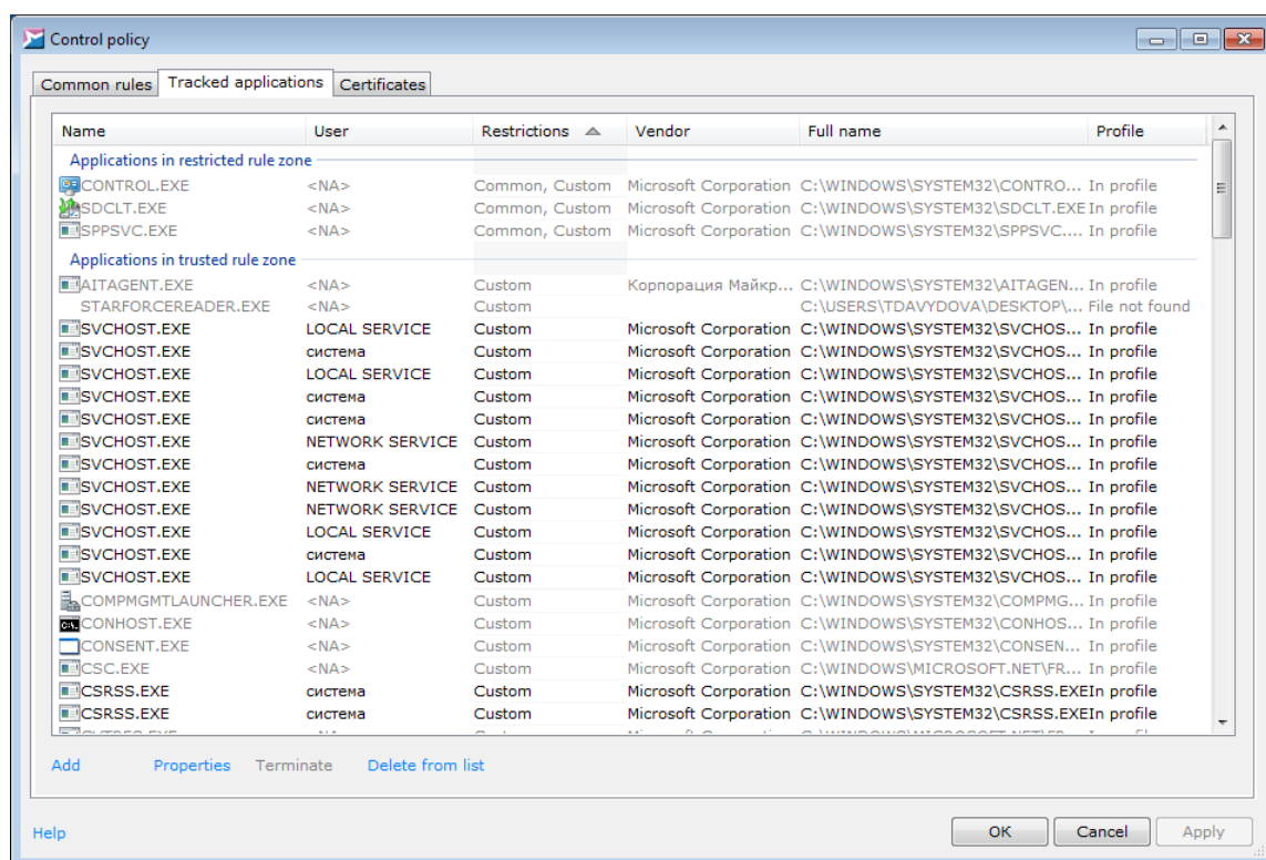
Figure 51. Tracked applications
