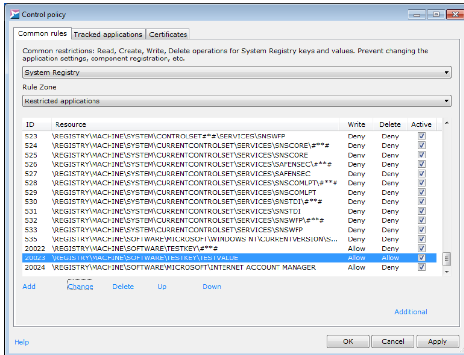
Figure 64. Control policy for the system registry
