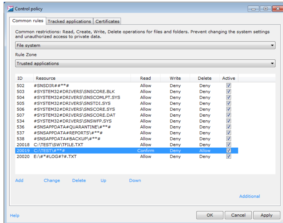
Figure 59. Control policy for the file system
