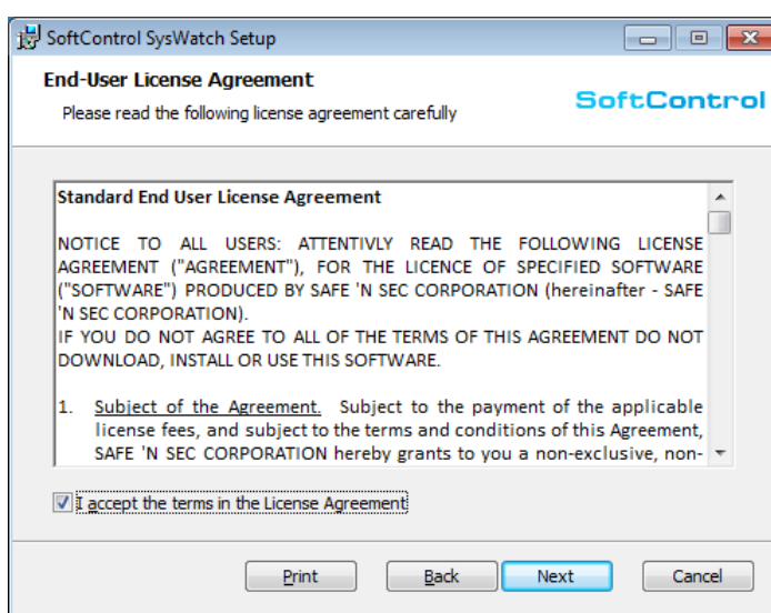
Figure 102. License agreement
