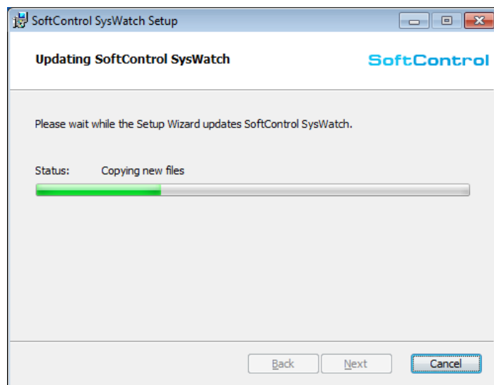
Figure 104. Updating progress
