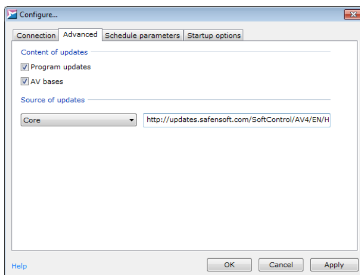
Figure 98. Selecting components to update
