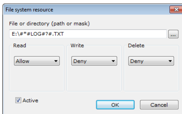
Figure 60. Creating a rule for the file system object
