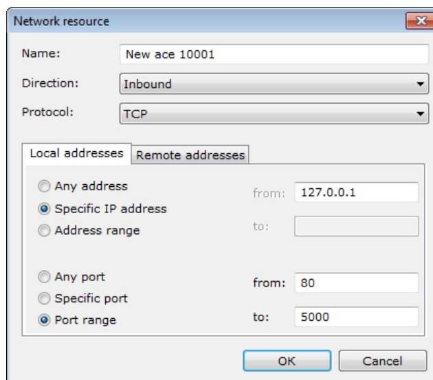
Figure 74. Creating a network activity rule
