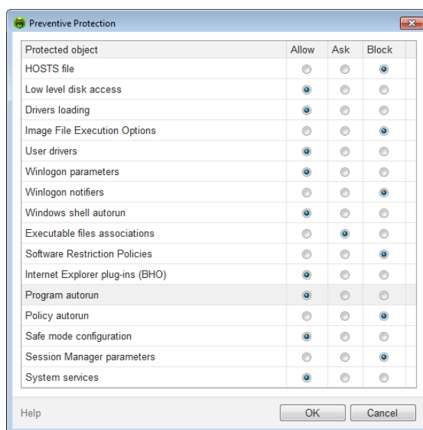
Figure 114. Custom settings for preventive protection
