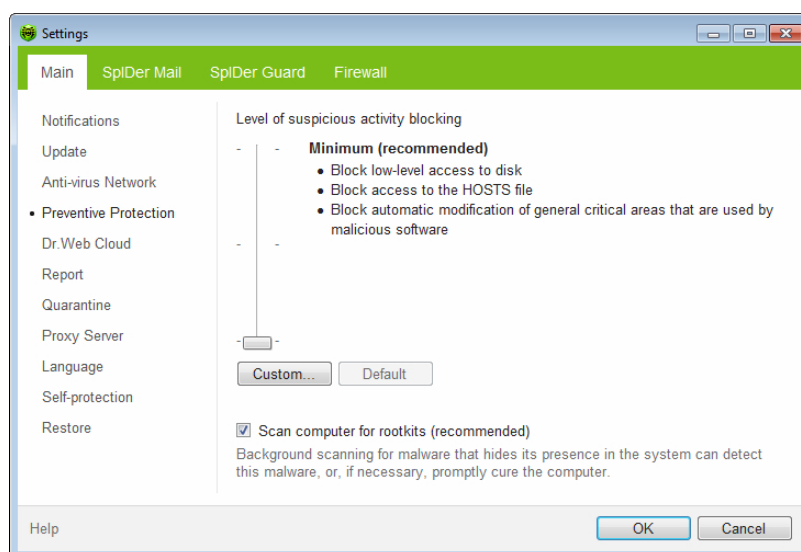
Figure 113. Preventive protection settings
