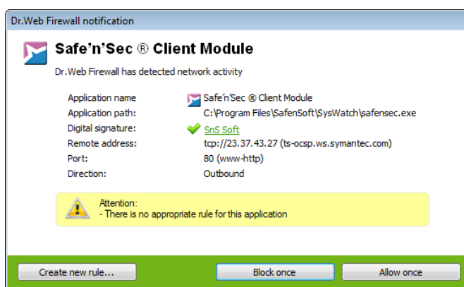
Figure 117. Dr.Web® Firewall notification
