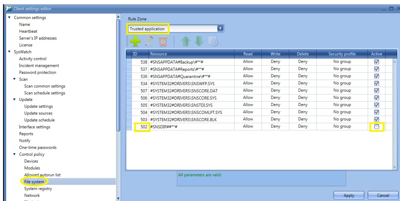
Figure 108. Uncheck rule 502 in client settings. Trusted applications
