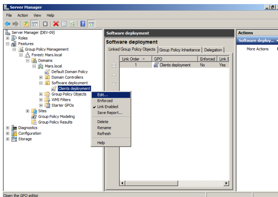
Figure 110. Modifying a group policy object
