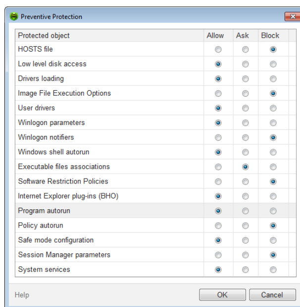
Figure 116. Custom settings for preventive protection
