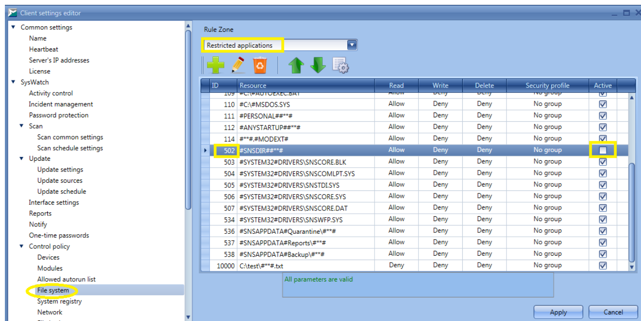
Figure 107. Uncheck rule 502 in client settings. Restricted applications
