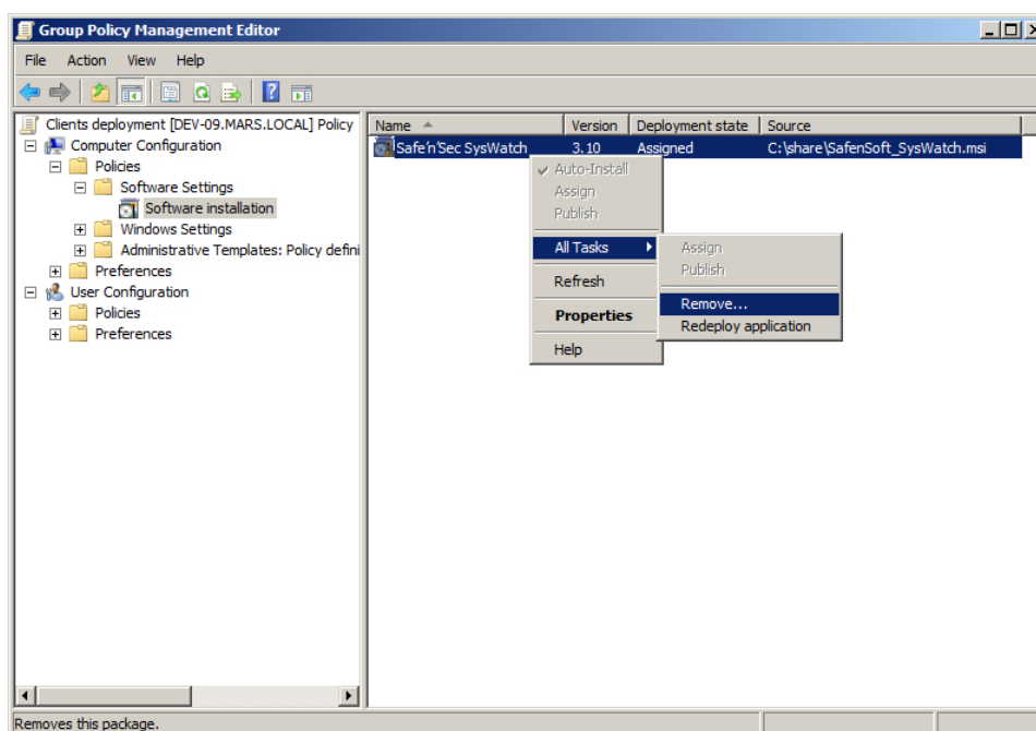
Figure 111. Invoking the application removal task
