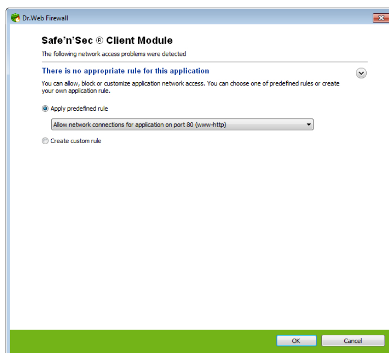
Figure 120. Creating a rule in Dr.Web® Firewall
