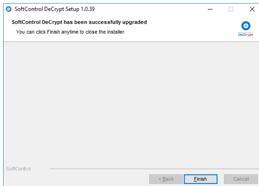
Figure 33. Update completes
