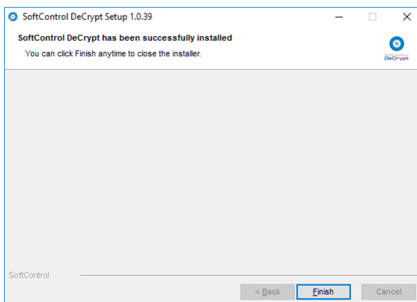
Figure 5. Installation completes
